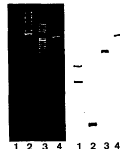
Figure 3. Confirmation of the EcoD recognition sequence. The plasmid pRSF 2124 was methylated with EcoD on a 4% polyacrylamide gel as described in the Legend to Figure 1. The left of the Figure shows the stained gel and the right the fluorogram. The type two restriction enzymes used were in lane 1, FnuDIII , lane 2 TaqI , lane 3 DdeI and lane 4 HaeII .
