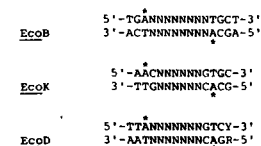
Figure 5. The recognition sequences of EcoK, EcoB and EcoD. The methylated adenosyl residues of the modified sites are indicated with asterisks.
