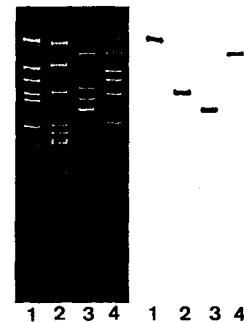
Figure 1. Mapping of the EcoD site in SV40 DNA. SV40 DNA was methylated in vitro with EcoD and 3 H-methyl AdoMet (Amersham, 64-72 Ci/mmol) as described (11). Labelled DNA was then cleaved with different type II restriction enzymes and the fragments were separated on a 4% polyacrylamide gel which was then stained with ethidium bromide and photographed, dried and fluorographed. The left panel shows the stained gel and the right panel the fluorogram. Lanes 1, RsaI digestion, a fragment extending from 1385-2989 is labelled; lanes 2, HaeIII digestion, label is in the fragment extending from 2177-2716; lanes 3, DdeI digestion, the coordinates of the labelled fragment are 2293-2710; lanes 4 show a BstNI digestion and a fragment extending from 1453-2445 is labelled.
