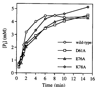
Figure 4. Time course of ATP hydrolysis by EcoAI mutants. 20 nM pJP25 DNA (a single EcoAI site) was incubated with 80 nM enzyme in buffer C at 37°C. During the incubation, 10 μl aliquots were removed and the reaction was stopped by the addition of 1 vol of 0.1 mM EDTA (pH 8). The concentration of inorganic phosphate ( P_i ) released by ATP hydrolysis was measured as described in Materials and Methods.
